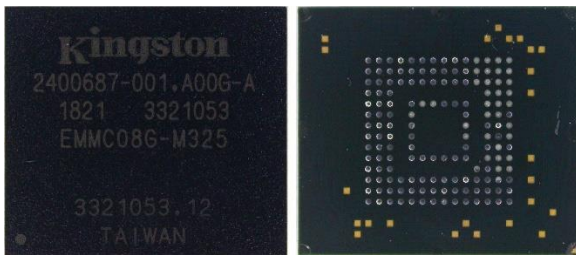
Fig. 65. Kingston EMMC08G-M325 from both sides
