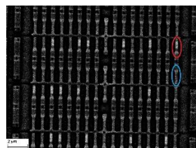
Fig. 73. Advanced contrast image of EEPROM in AT98SC008CT
