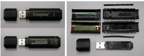
Fig. 27. DataTraveler DT4000G2 before and after opening its plastic case
