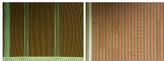
Fig. 72. Mask ROM data visible under optical microscope in AT90SC chip
