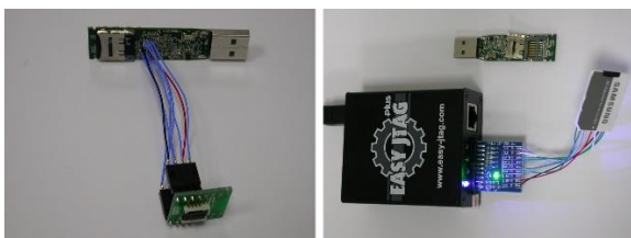
Fig. 61. Testing Serial Flash and microSD card from IronKey F150
