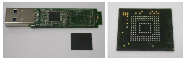
Fig. 63. Testing eMMC Flash from DataTraveler DT4000G2
