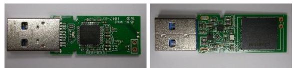
Fig. 33. PCB image of DataTraveler Locker+G3
