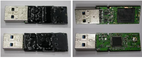
Fig. 51. Integral Crypto before and after epoxy removal
