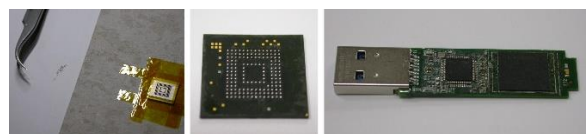
Fig. 64. Soldering eMMC Flash back to PCB of DataTraveler DT4000G2
