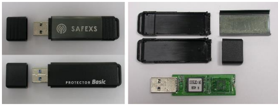
Fig. 59. SafeXS Protector before and after opening its plastic case
