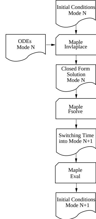
Fig. 3. Determining the Closed Form Solutions for Each Mode
