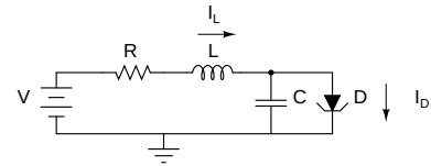
Fig. 5. Tunnel Diode Oscillator
