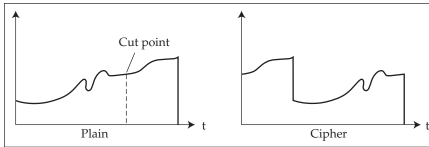
Figure 24.1: Cut-and-rotate scrambling
